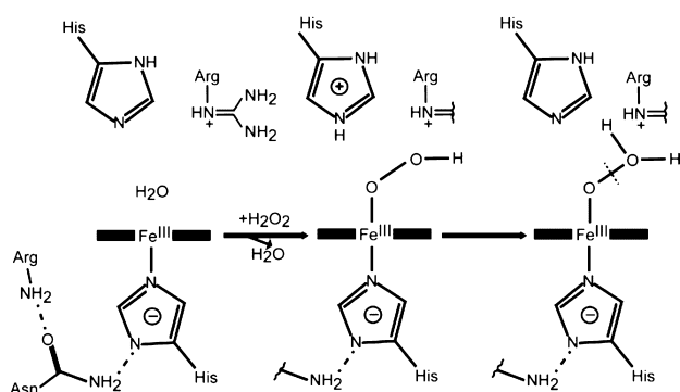
Figure 2. Mechanism of Compound 0 formation in LPO.
