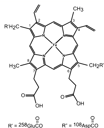
Figure 1. Scheme of heme I in LPO.
